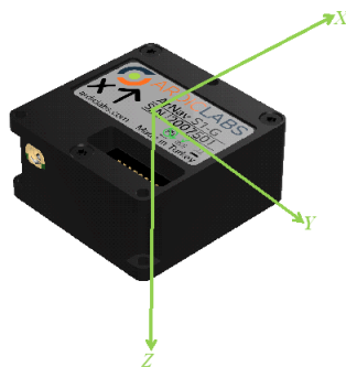
Figure 7: ArNav body coordinate system
