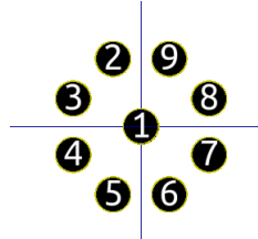
Figure 13: ArNav M2 Auxiliary Connector Pin Positions, Front View
